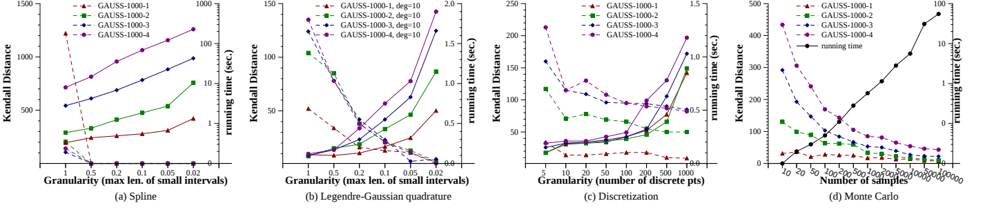
Figure 7: The comparison of various methods for computing PRF^e ( \epsilon = 0.99 ). Solid lines indicate the running times (with axes drawn on the right hand side), whereas dashed lines indicate the Kendall distance (an error measure).
