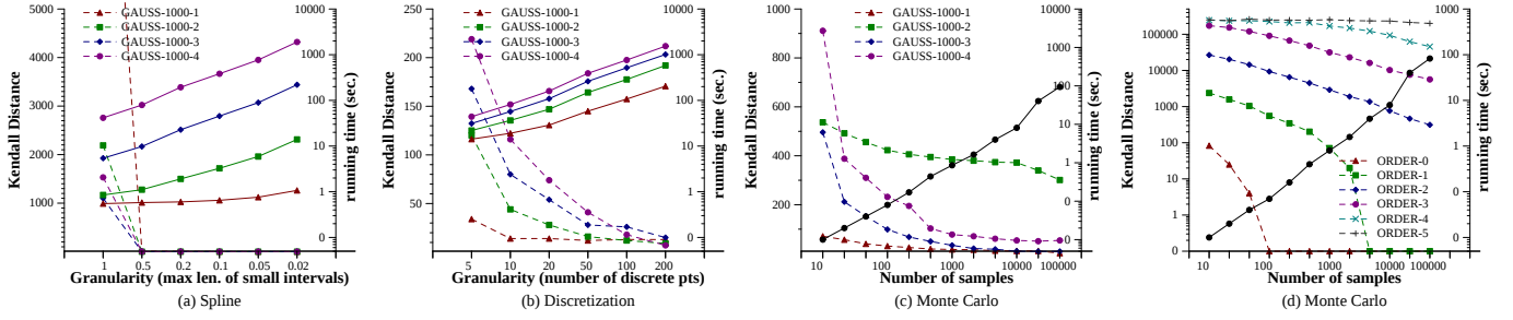
Figure 5: The comparison of various methods for computing general PRF (weight function !(t; j) = 1=j ). Solid lines indicate the running times (with axes drawn on the right hand side), whereas dashed lines indicate the Kendall distance (an error measure).
