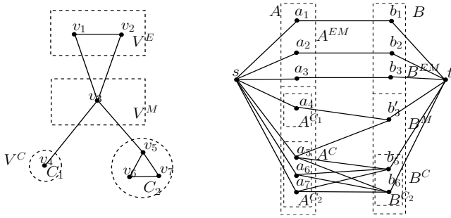
Figure 1: The left hand side illustrates the the Gallai-Edmonds decomposition of the graph and the right hand side is the corresponding flow network.
